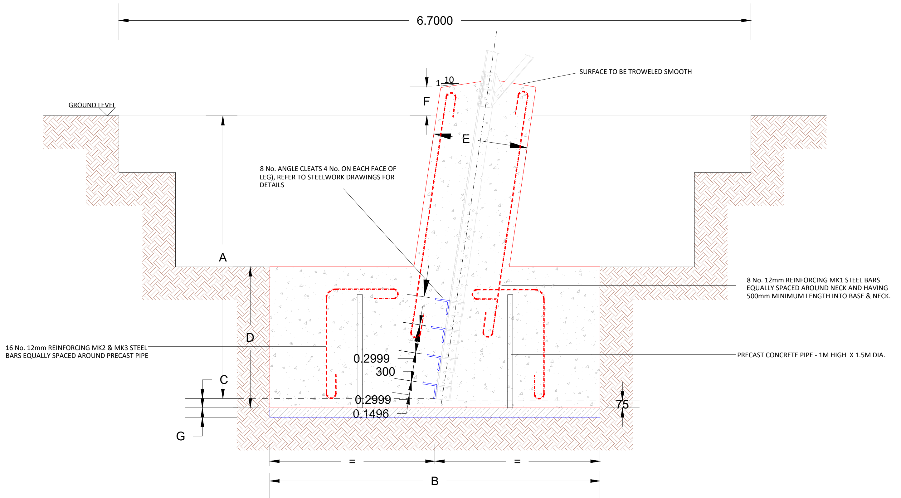
FOUNDATION ELEVATION SECTION
