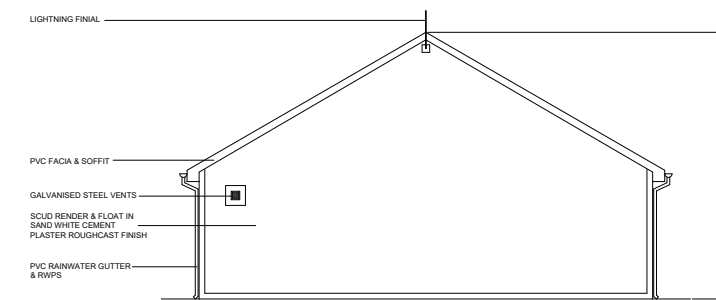
SECTION VIEW D - D
