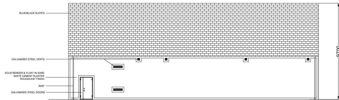
SECTION VIEW B - B
