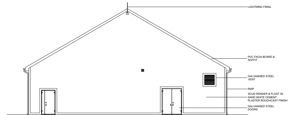
SECTION VIEW C - C
