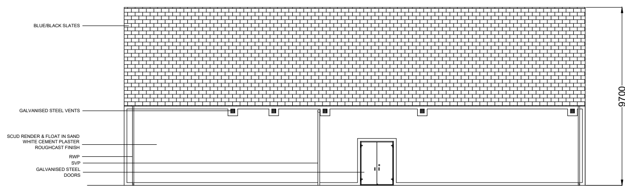
SECTION VIEW A - A
