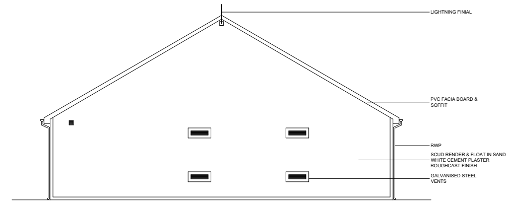
SECTION VIEW D - D
